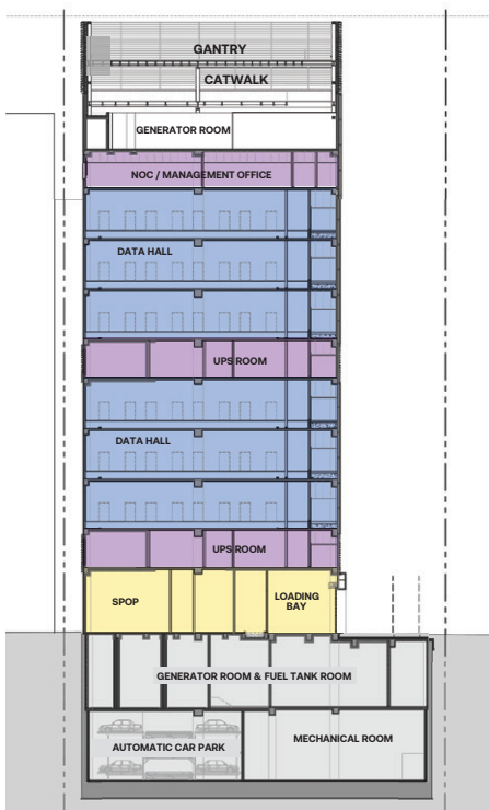
Program Zoning Section
