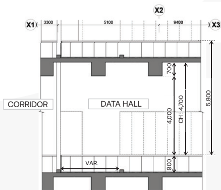
Standard Data Hall Section
